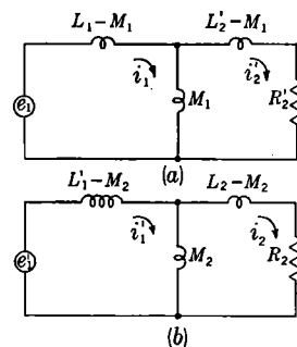
FIG. 12-4.—Circuits equivalent to those shown in Fig. 12-3.
